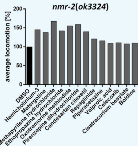
Movement score average over 600 minutes in nmr-2(ok3324) mutants relative to DMSO controls.
